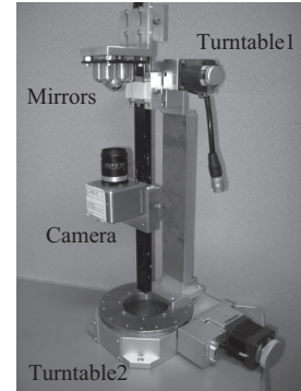
Fig. 4. Experimental calibration system with two turntables.
