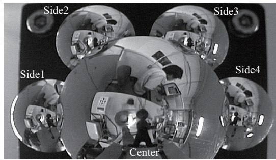
Fig. 5. Example of the image of compound parabolic mirrors.
