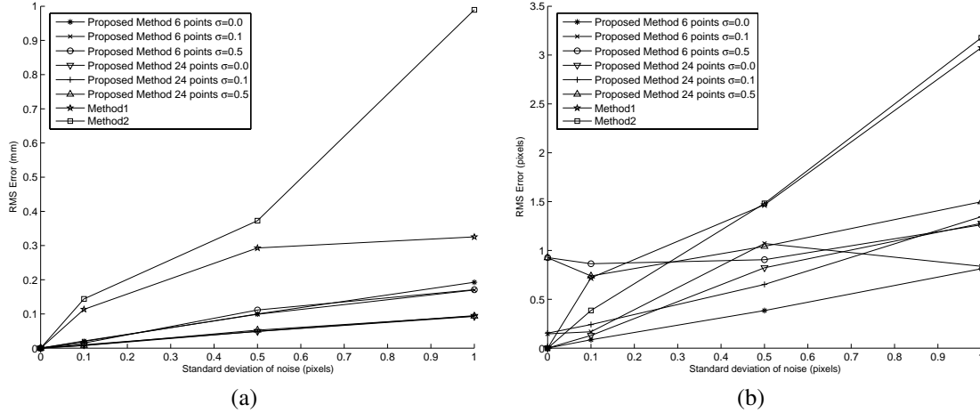
Fig. 3. Error in estimating the mirror position: (a) RMS error of the translation. (b) RMS error of the reprojected points.
