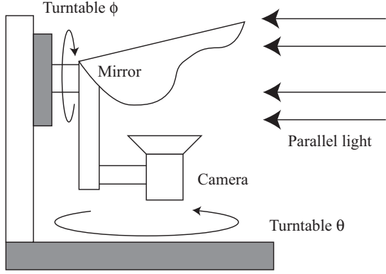
Fig. 2. Calibration system using parallel lights: The camera and mirror is rotated by two turntables.
