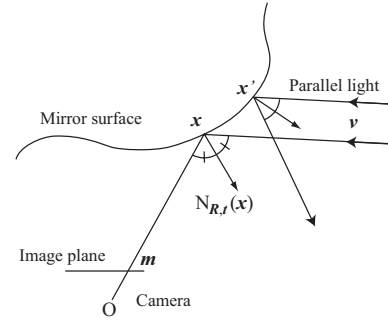
Fig. 1. Projecting a parallel light to a catadioptric imaging system.
